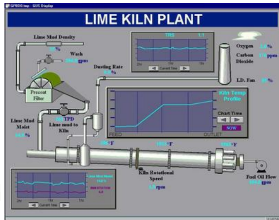
Figure 22- Lime Kiln Process P&ID [25]
