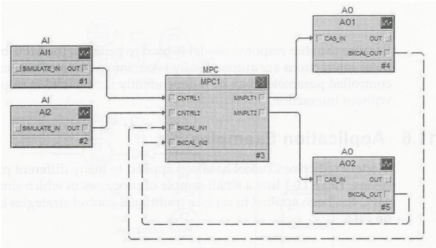
Figure 2 - MPC Implementation for Interactive Processes [25]
