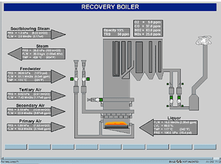
Figure 3- Recovery Boiler DCS Operator Graphic
