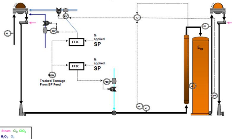
Figure 20- E OP Control [22]
