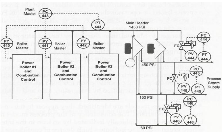
Figure 4- Powerhouse Plant Master [25]
