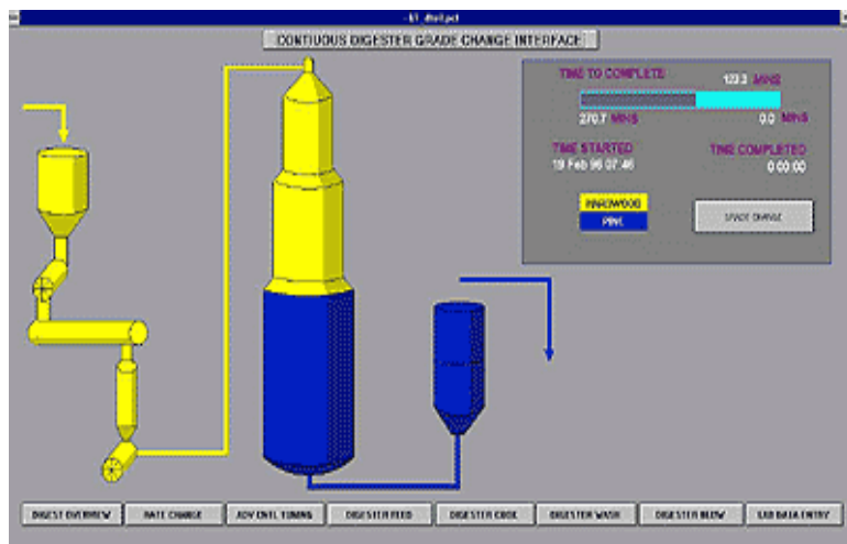
Figure 14- Continuous Digester Grade Change
