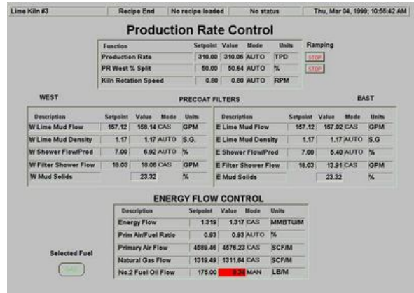
Figure 26- Lime Kiln Production Rate Control
