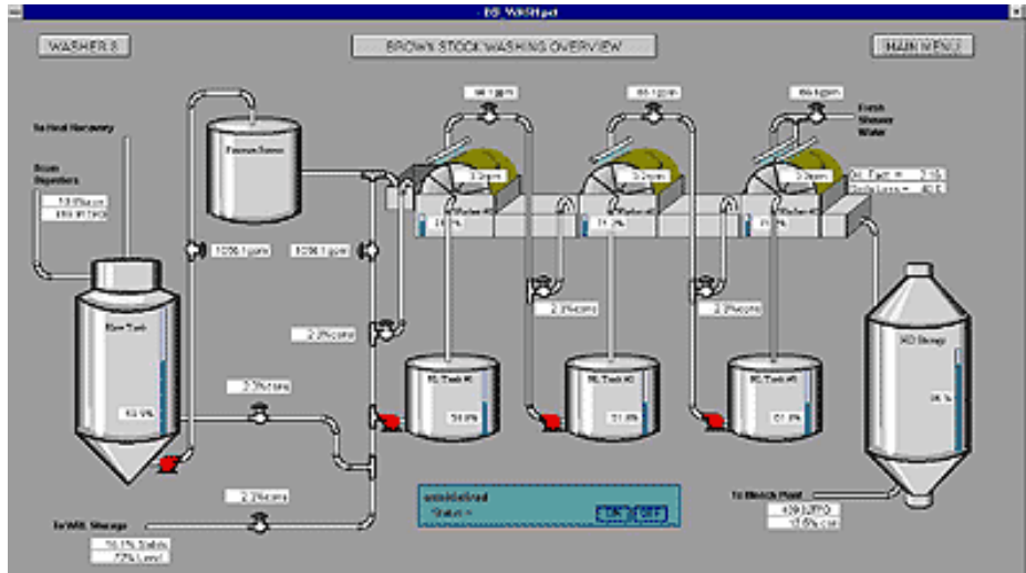
Figure 17- Brown Stock Washer Overview
