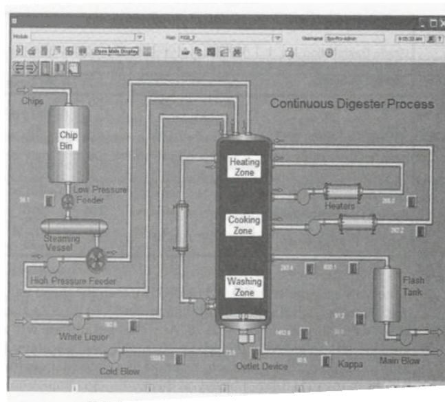
Figure 12- Continuous Digester DCS Operator Graphic [25]
